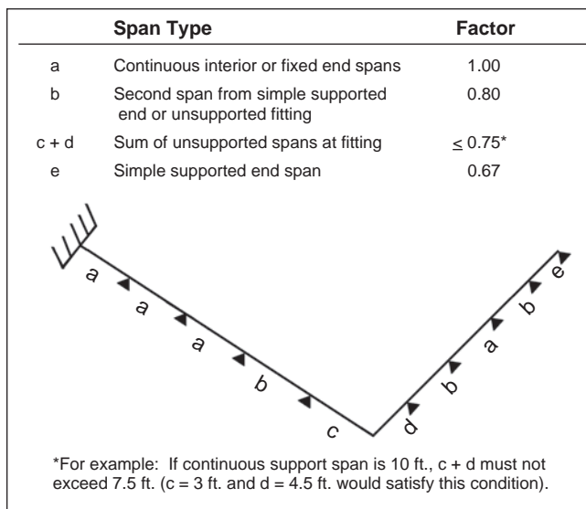
Figure 2.13 Piping Span Adjustment Factors With Unsupported Fitting at Change in Direction
